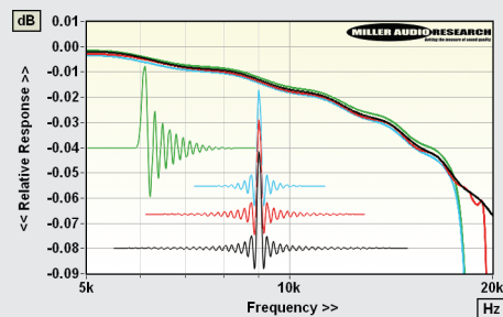
ABOVE: Treble (zoomed, 5kHz-20kHz) and impulse resps. for Mytek Brooklyn DAC via Aries G2.2 (Precise, black; Dynamic, red; Balance, blue; Smooth, green)
